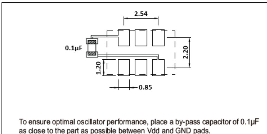
Pad Layout mm shown
