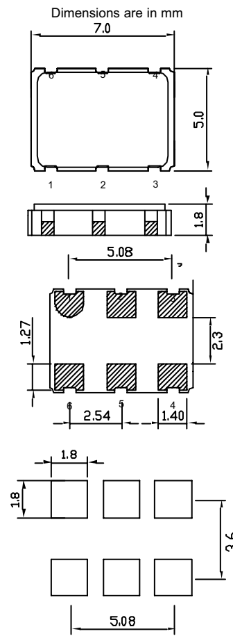
Solder Pad Layout
